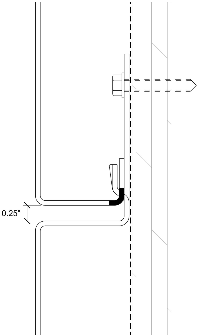
A-A Section - Panels on Continuous Substrate
