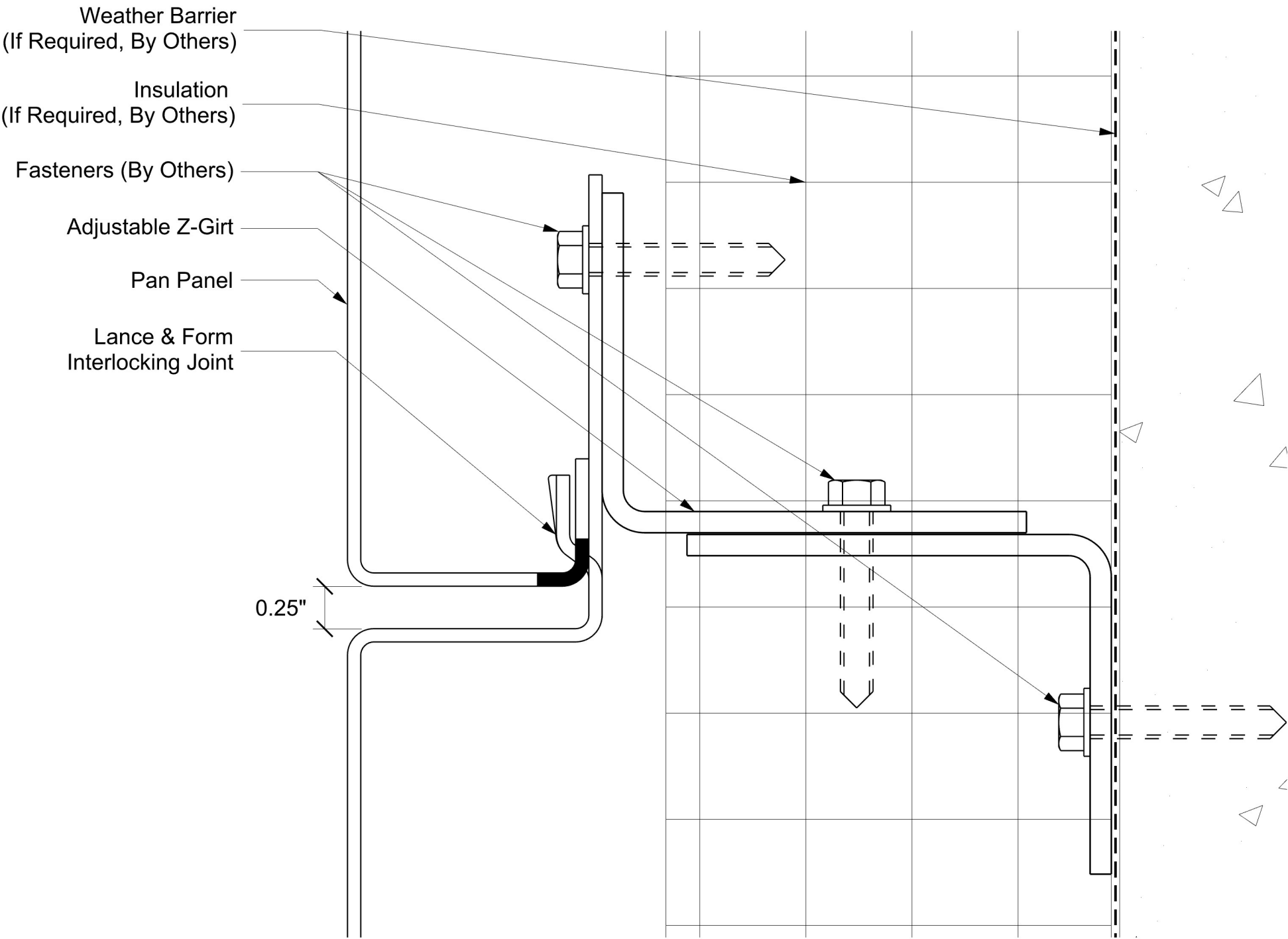
A-A Section - Panels on Adjustable Z-Girt
