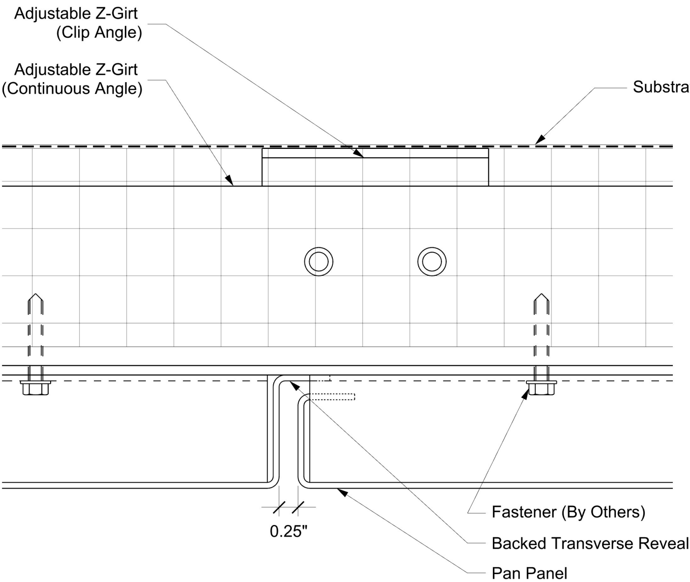
B-B Section - Panels on Adjustable Z-Girts
